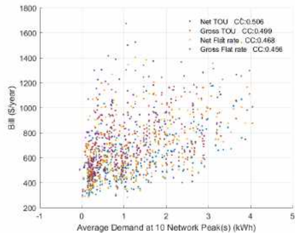
Fig. 3 Tariff impact analysis for case study 1: scatter plot of bill versus demand of customers in top 10 network peaks
