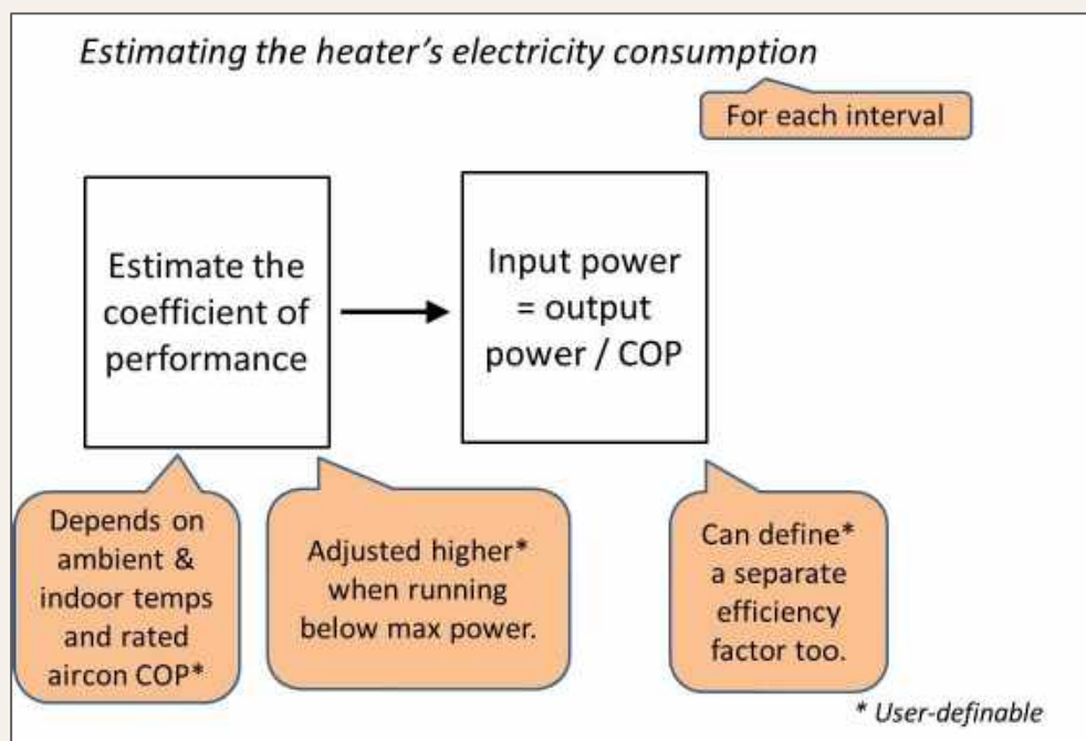
Figure 16 Flow Chart Logic, Air Conditioning Energy Usage (2)
