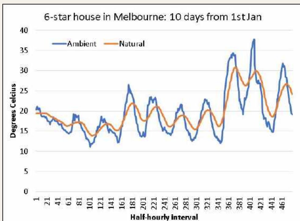
Figure 13 Moving Average of the Ambient versus Natural Indoor Air Temperature
