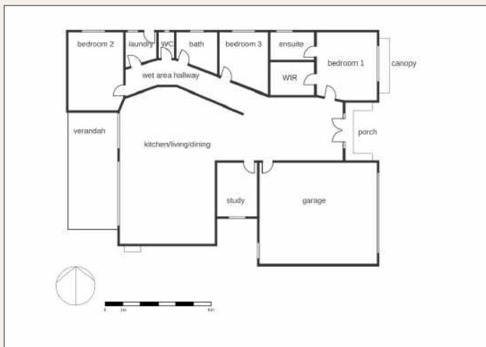
Figure 12 Floor Plan, BZE Reference Home (Medium Home Size Modelled)
