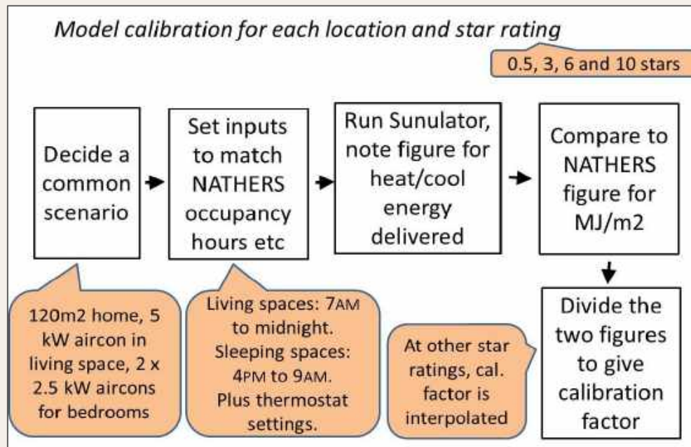
Figure 17 Flow Chart Logic, Calibration against NatHERS
