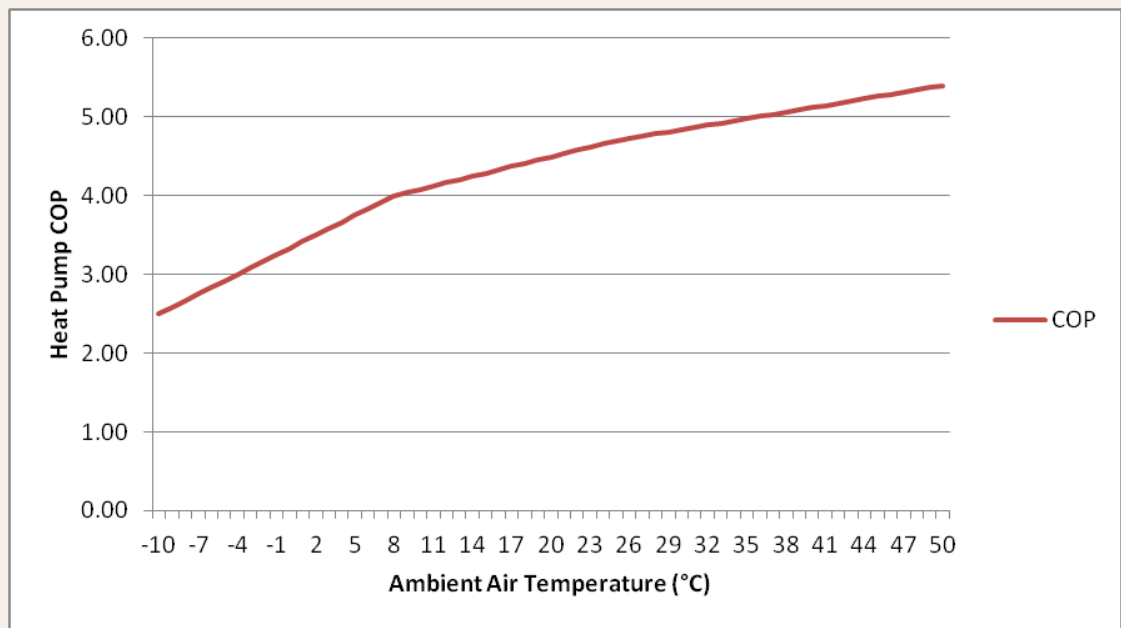
Figure 19 Impact of Ambient Air Temperature on Heat Pump COP
