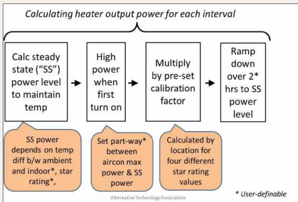
Figure 15 Flow Chart Logic, Air Conditioning Energy Usage (1)
