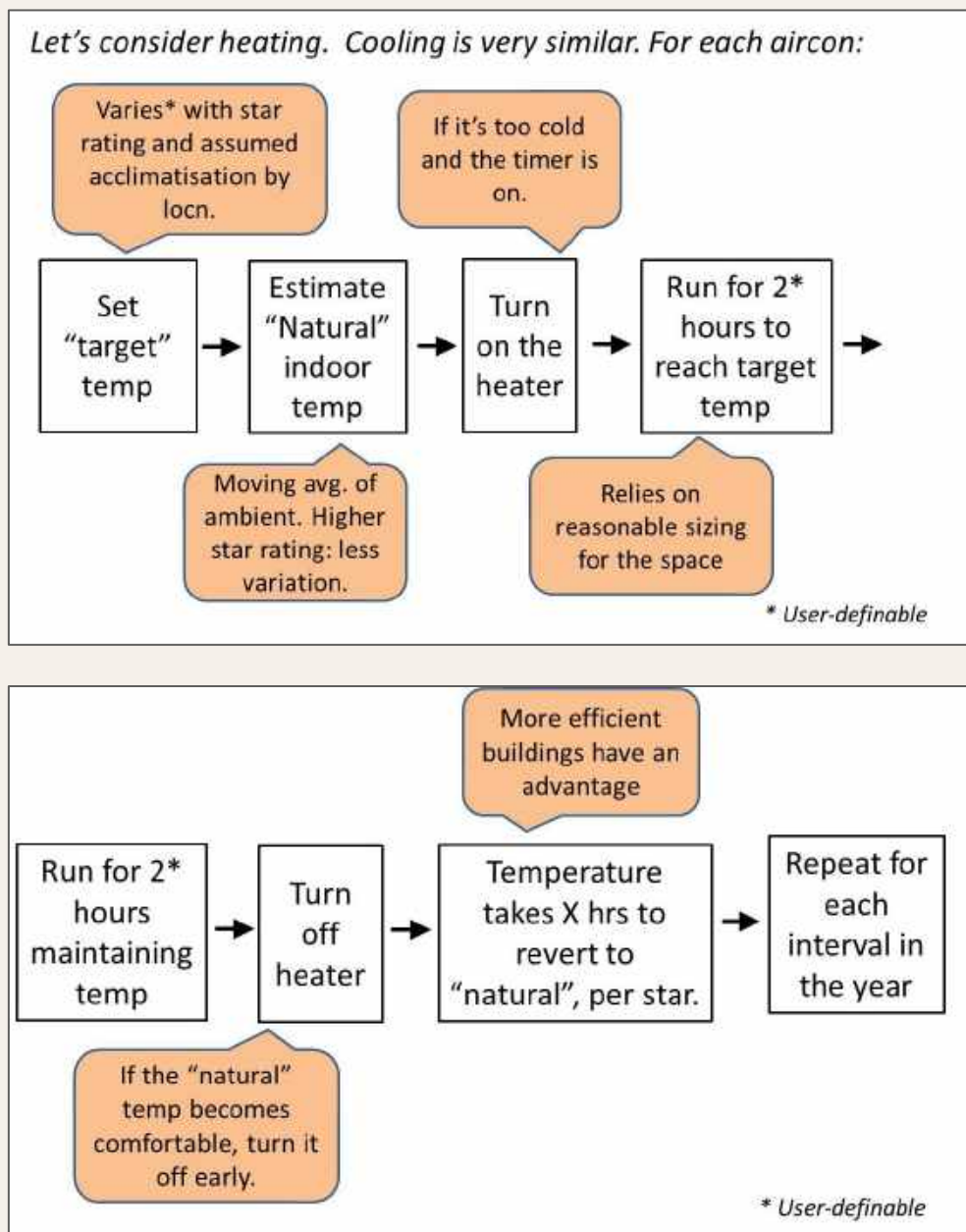
Figure 14 Flow Chart Logic, Air Conditioning Control
