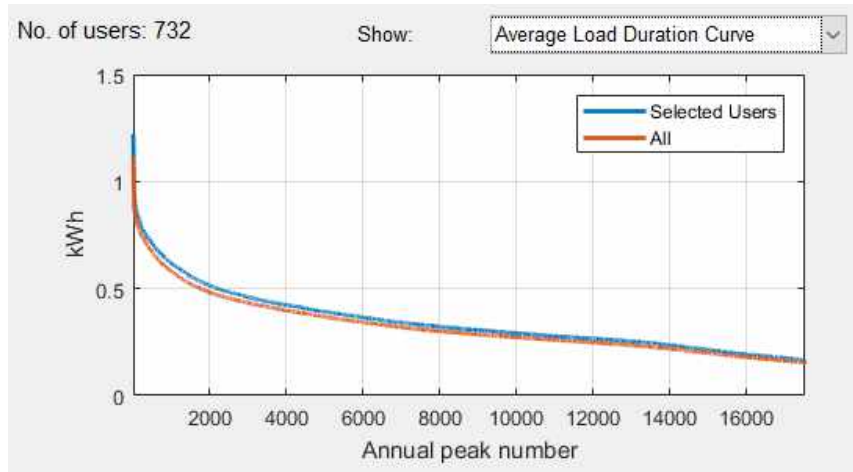
Figure 7 Average Load Duration Curve (sorted aggregate load profile in kW in descending order)
