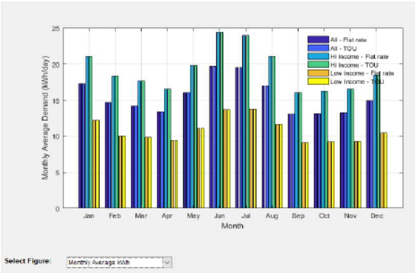
Figure 21 Monthly Average kWh
