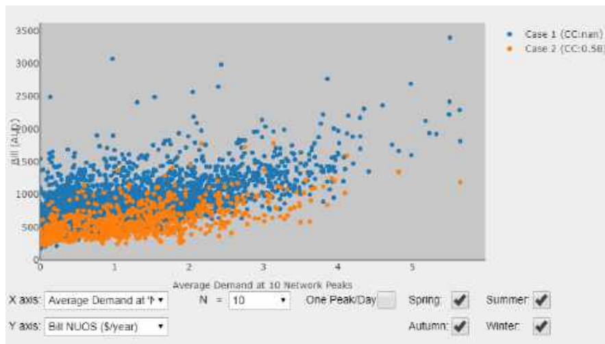
Figure 51 NUOS component of the Bill vs Average demand at the times of network peak
