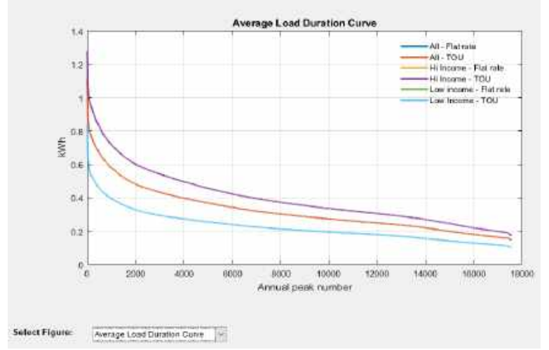
Figure 24 Average Load Duration Curve
