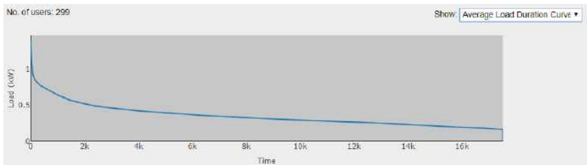
Figure 35 Average Load Duration Curve (sorted aggregate load profile in kW in descending order)
