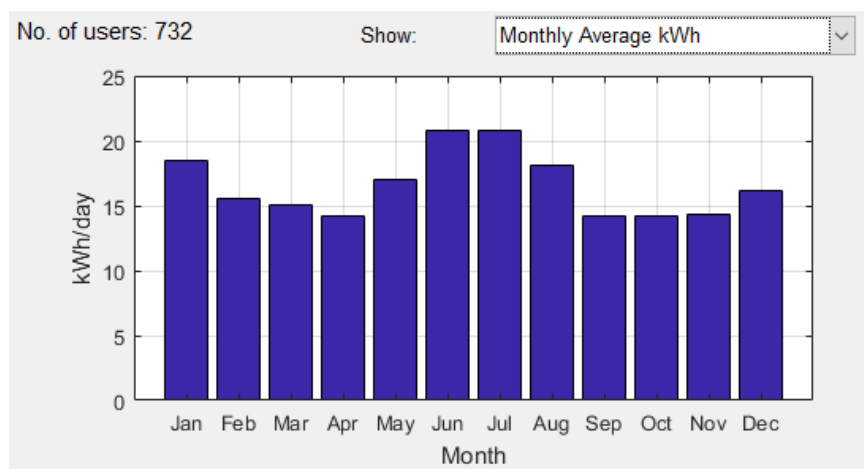
Figure 9 Monthly Average kWh
