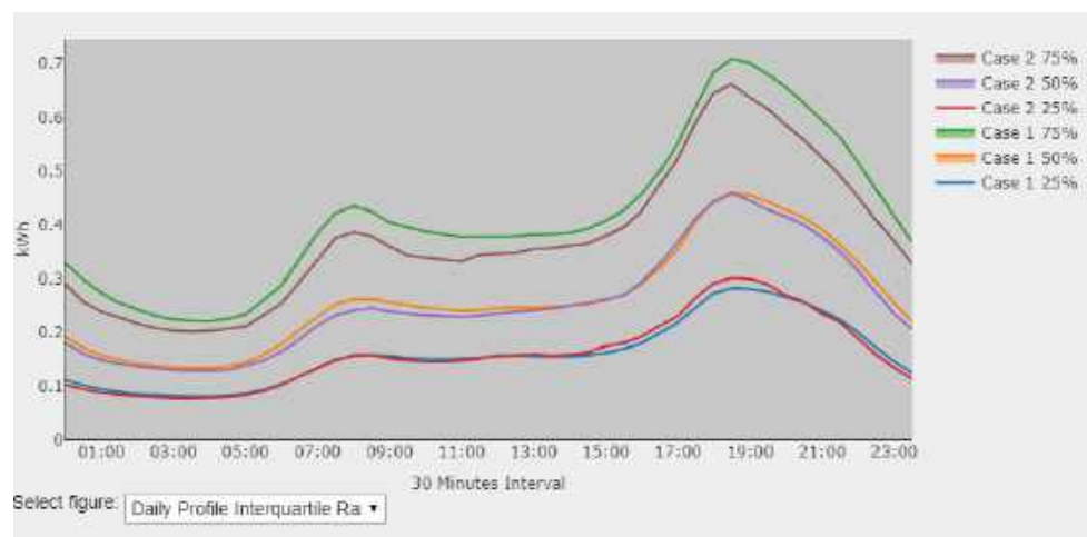
Figure 48 Interquartile range of the load profiles in two case studies
