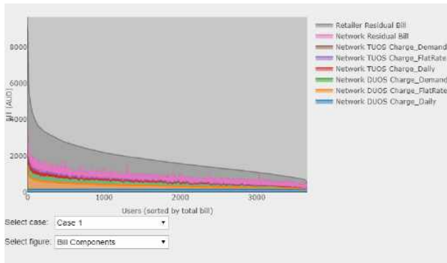
Figure 52 contribution of different components to the total bill for all customers (sorted by the total bill of customers)
