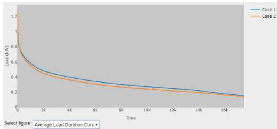
Figure 46 Load duration curves of two sample case studies
