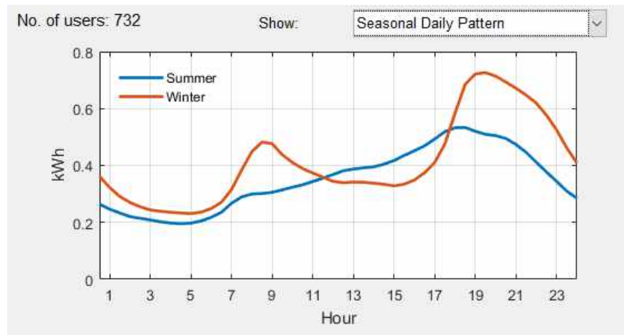
Figure 10 Seasonal Daily Pattern (average daily load pattern in summer and winter months)
