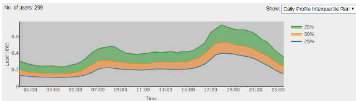
Figure 33 Daily Profile Interquartile Range (25%, 50%, and 75% of load)
