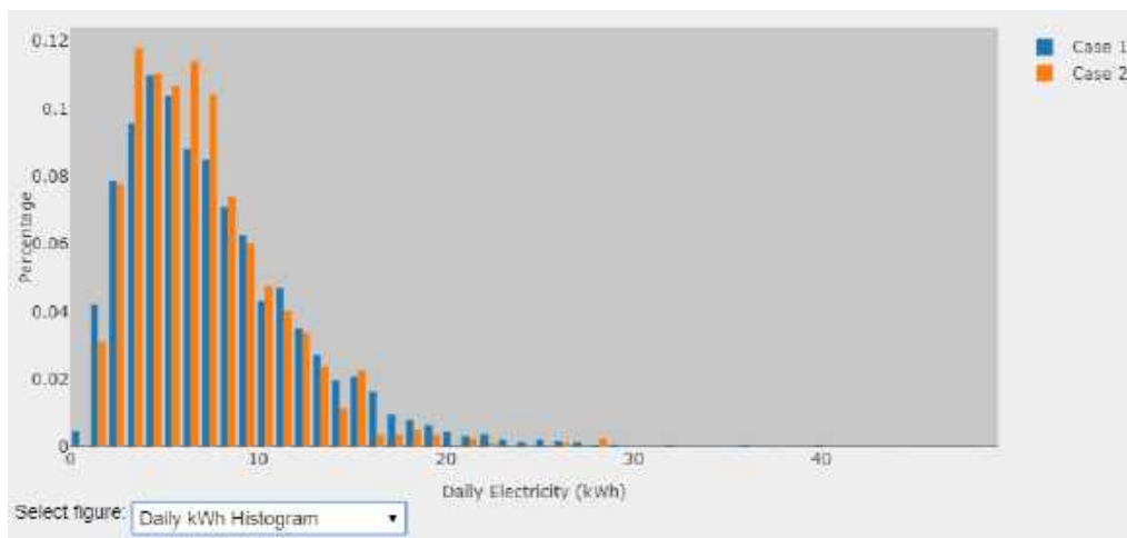
Figure 45 Histogram of the kWh in two sample case studies
