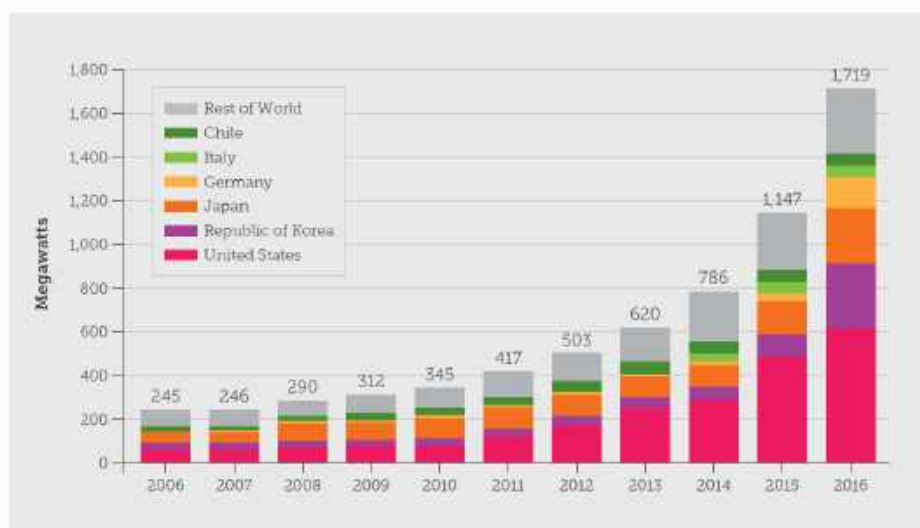
Figure 10: Global grid-connected battery storage capacity by country, 2005-2016
