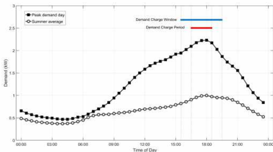
Figure 13. Summer Peak and Average Demand Days, with Demand charge Window and Period
