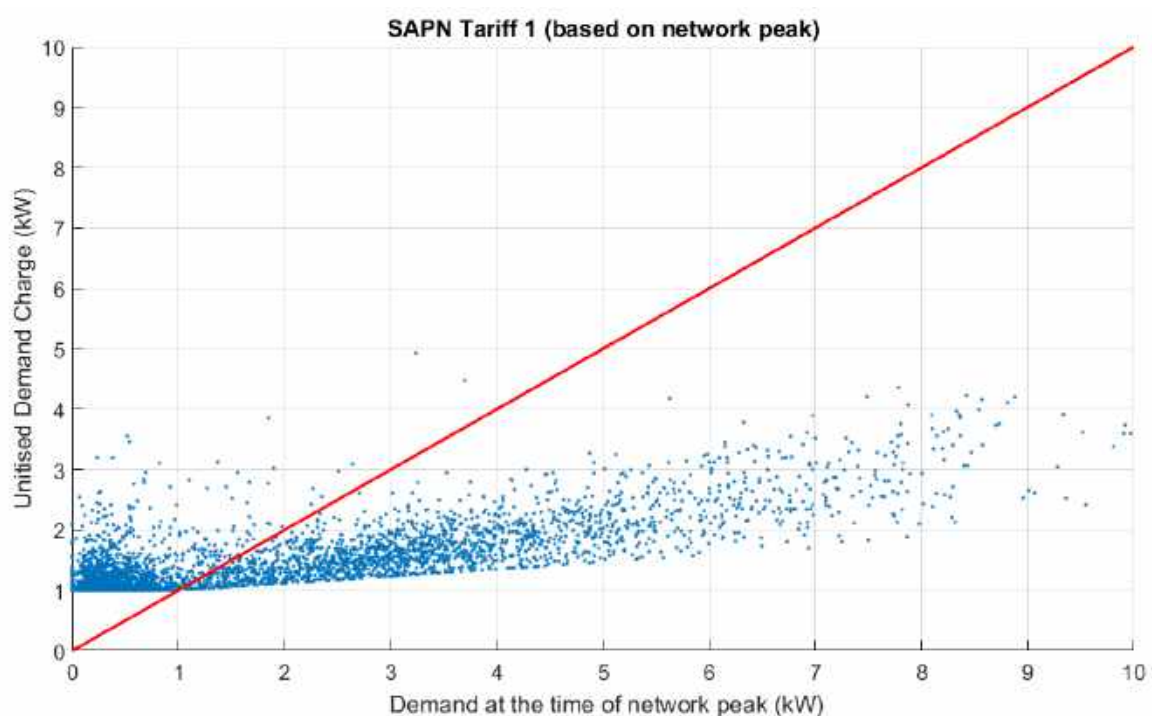
Figure 7. Unites Demand Charge based on Customer Demand at Time of Network Peak vs Demand at Time of Network Peak – only summer and winter months
