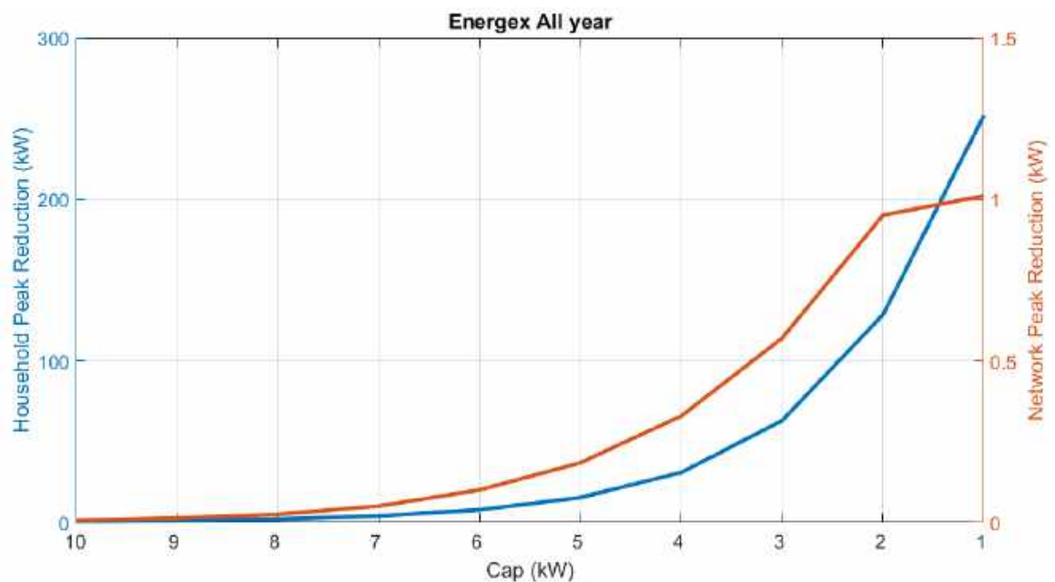
Figure 5. Household Peak Reduction vs Network Peak Reduction - Energex
