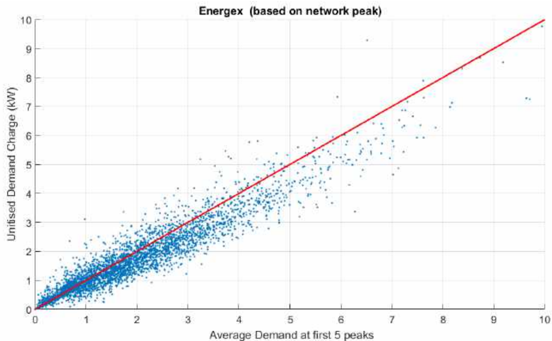
Figure 15. Unitised Demand Charge based on Customer Demand at Time of Network Peak vs Average Demand at Time of 5 Highest Network Peaks – only summer and winter months - Energenx
