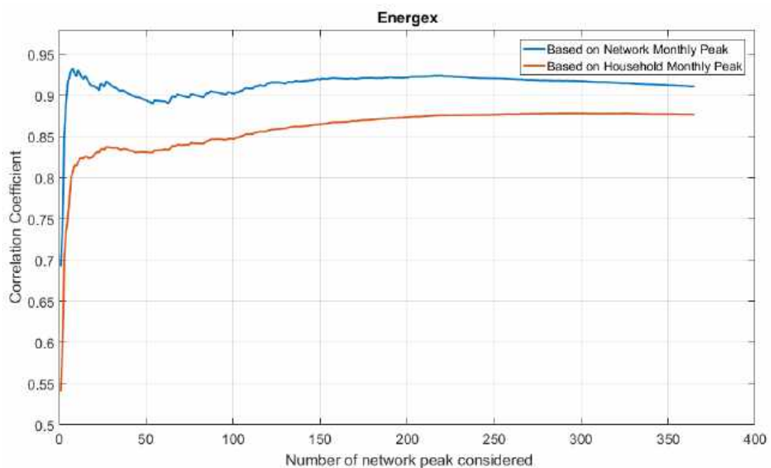
Figure 9. Impact on Correlation Coefficient of Increasing the Number of Peak Days - Energen
