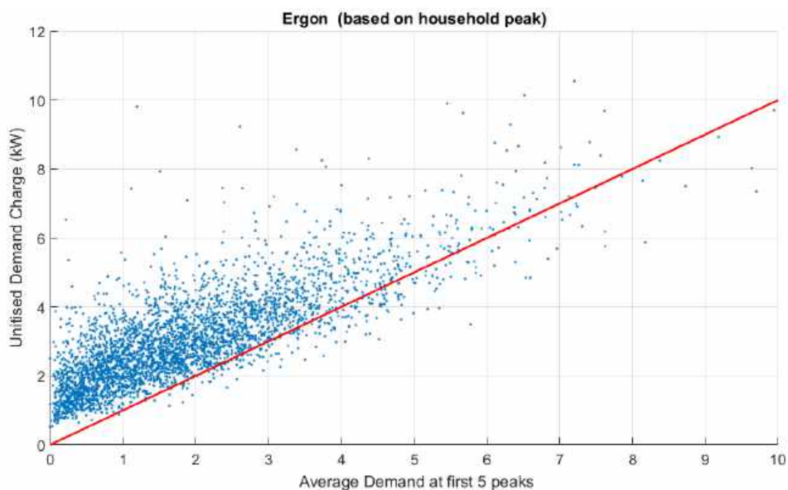
Figure 16. Unitised Demand Charge vs Average Demand at Time of 5 Highest Network Peaks – Ergon's standard demand tariff
