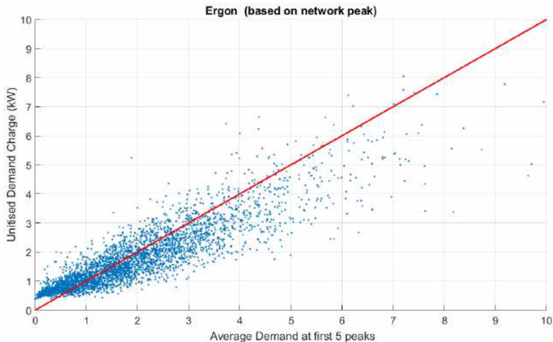
Figure 18. Unifised Demand Charge based on Customer Demand at Time of Network Peak vs Average Demand at Time of 5 Highest Network Peaks – only summer and winter months, with min 3kW charge removed - Ergon
