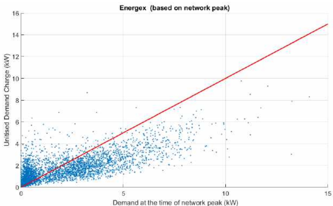
Figure 13. Unitised Demand Charge based on Customer Demand at Time of Network Peak vs Demand at Time of Network Peak – Energex optimised tariff
