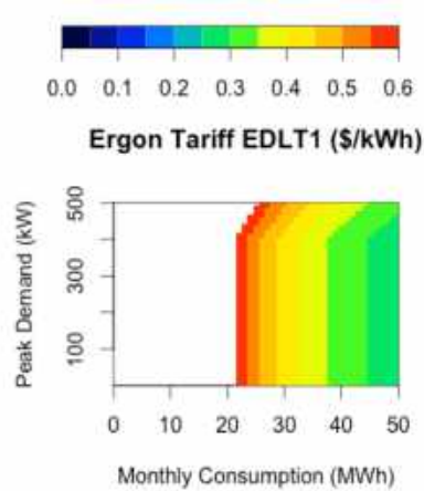
Figure 8. Ergon Tariff EDLT1 Average Price (Threshold Demand 400kW) MWh per month
