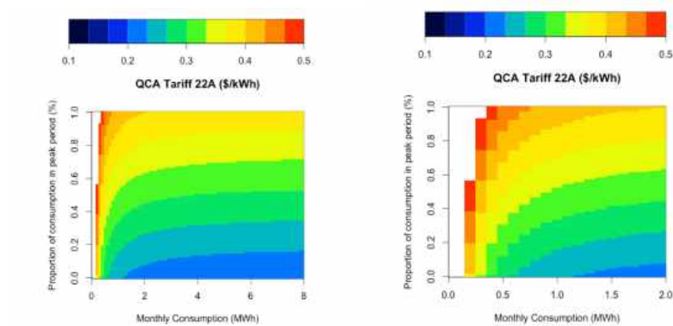
Figure 21. QCA Tariff 22A (a) 0 - 8 MWh per month (b) 0 - 2 MWh per month
