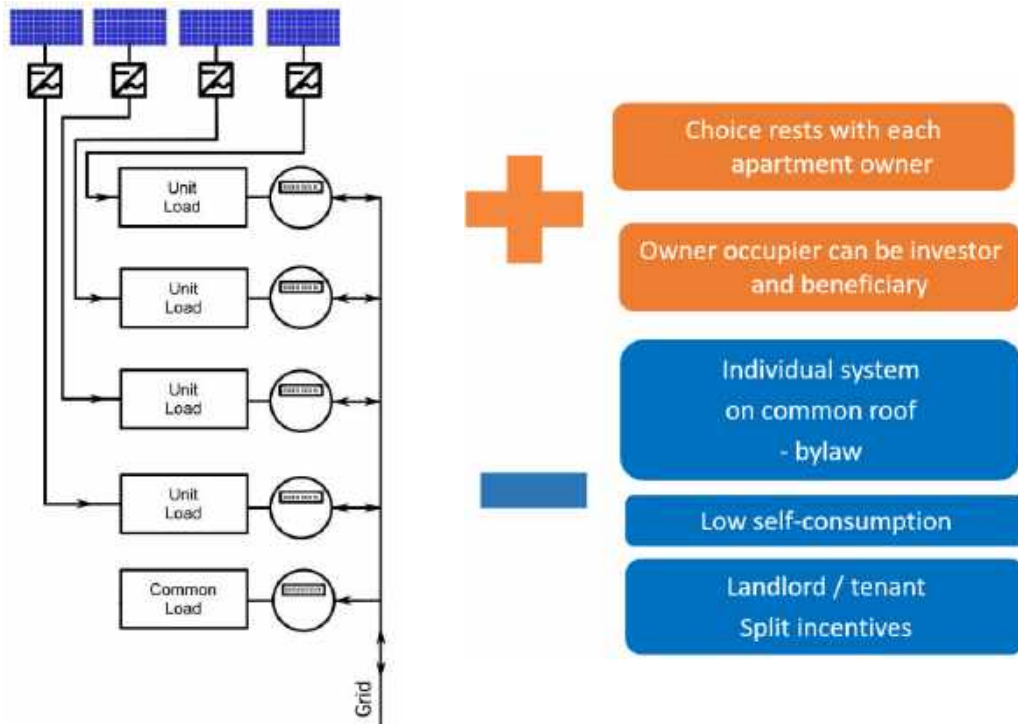
Figure 8 Individual PV for apartments
